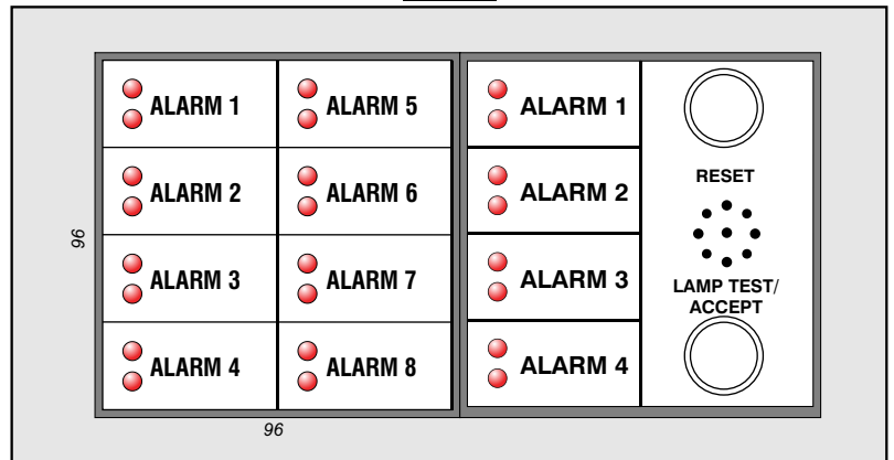
FRONT BEZEL (96x192mm) PANEL CUT-OUT (92x188mm)
