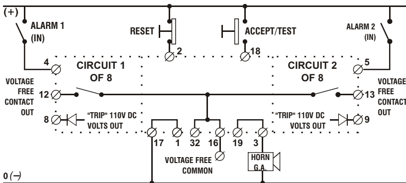
ADDA 8 - TYPICAL CONNECTION (ABOVE DIAG. IS FOR 2 OUT OF 8 ALARMS)
