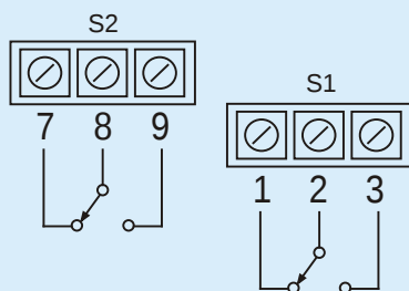
DigiRail - 2R Relay Output
