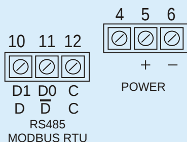
Communication and Power (for all models)
