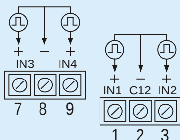
DigiRail - 4C Digital Inputs
