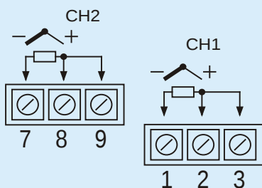
DigiRail - 2A Analog Inputs
