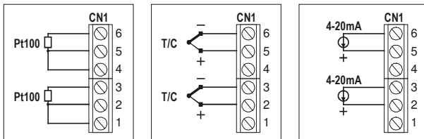
Figure 09 – Input signal connections
